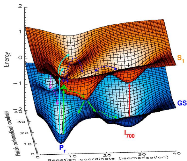
FIGURE 9 Cartoon showing a three-dimensional presentation of the excited ( S_1 ) and ground state (GS) potential energy surfaces for the P_r to P_{rf} phototransformation of native phyA. The S_1 potential surface of P_r has several potential minima which are separated by low barriers and can be reached after photoexcitation. The model separates the reaction coordinate for chromophore isomerization from the perpendicular reaction coordinate(s) of the protein/chromophore conformations not leading to isomerization. The green arrows indicate the excitation into a state with low excess energy and direct relaxation into the active channel leading to I_{700} . The green shaded Gaussian (reached by the green upward arrow from P_r ) indicates the initially created wavepacket in the excited state. The light blue arrows show excitation into states with higher excess energy. The dark blue arrows show movements on the excited-state potential surface—involving chromophore and protein modes—leading out of nonreactive or less reactive channels (potential minima). The red arrow indicates excitation of I_{700} into an excited-state surface common to I_{700} and P_r . The purple arrows indicate internal conversion from nonreactive potential minima back to the P_r ground state (for further discussion see text). Note that the detailed form of these potential energy surfaces should not be taken literally. The figure merely serves to illustrate the principal properties of the dynamics in the excited state and the interpretation of parallel and/or alternative processes.
