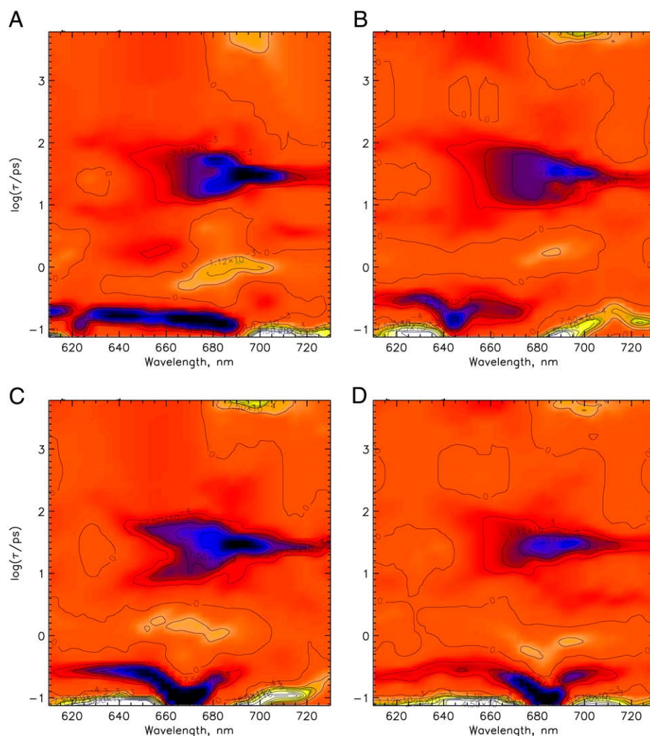
FIGURE 3 The lifetime density maps showing the excitation wavelength dependence of the femto- to nanosecond kinetics for native phyA in its P_r form. Excitation wavelengths are 620 nm (A), 640 nm (B), 665 nm (C), and 685 nm (D). Dark-blue color indicates negative and green/yellow-white positive amplitudes of a lifetime component while orange color reflects the zero level. The lifetime range is drawn on a logarithmic scale and extends from \sim 100 fs to \sim 6 ns (see Materials and Methods).
